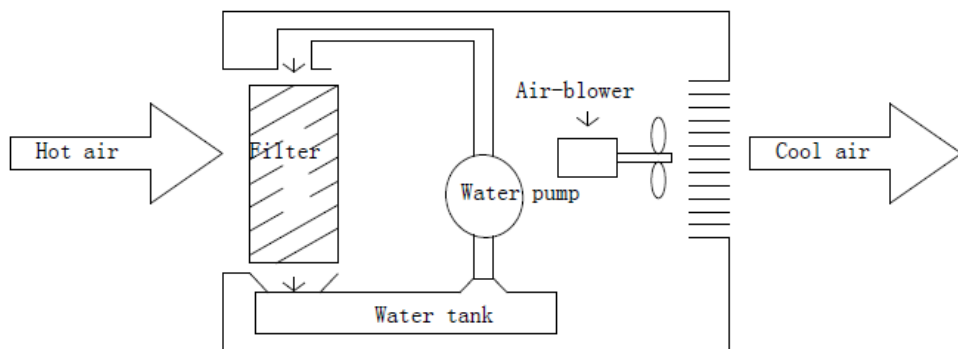
Principle Diagram
