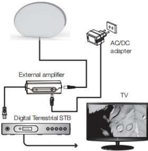
Digital TV Antenna
