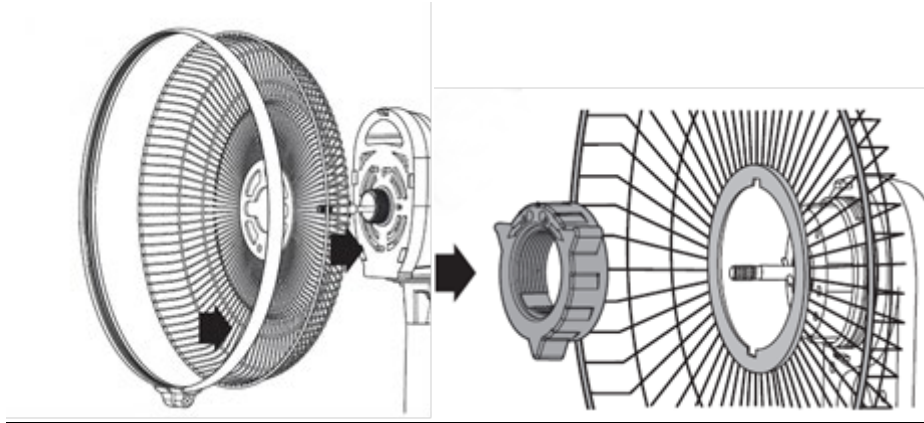
Fig. 1 – Locating lugs and locking nut
