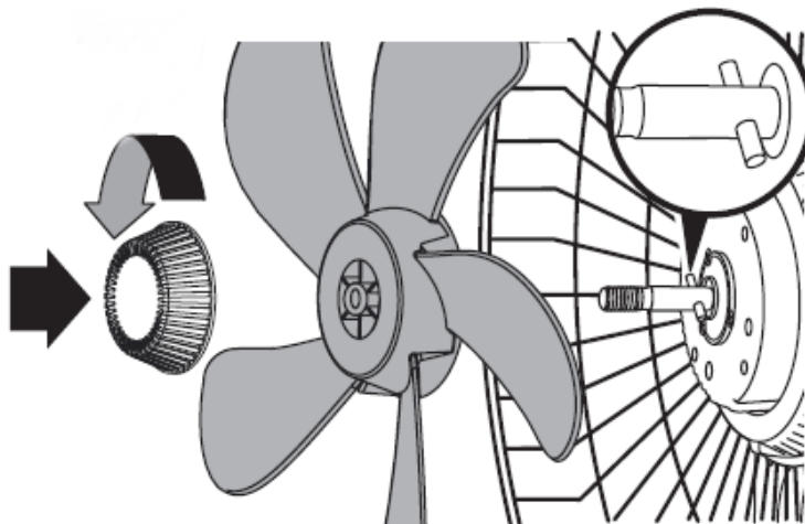
Fig. 2 – Motor Shaft tightens anti-clockwise
